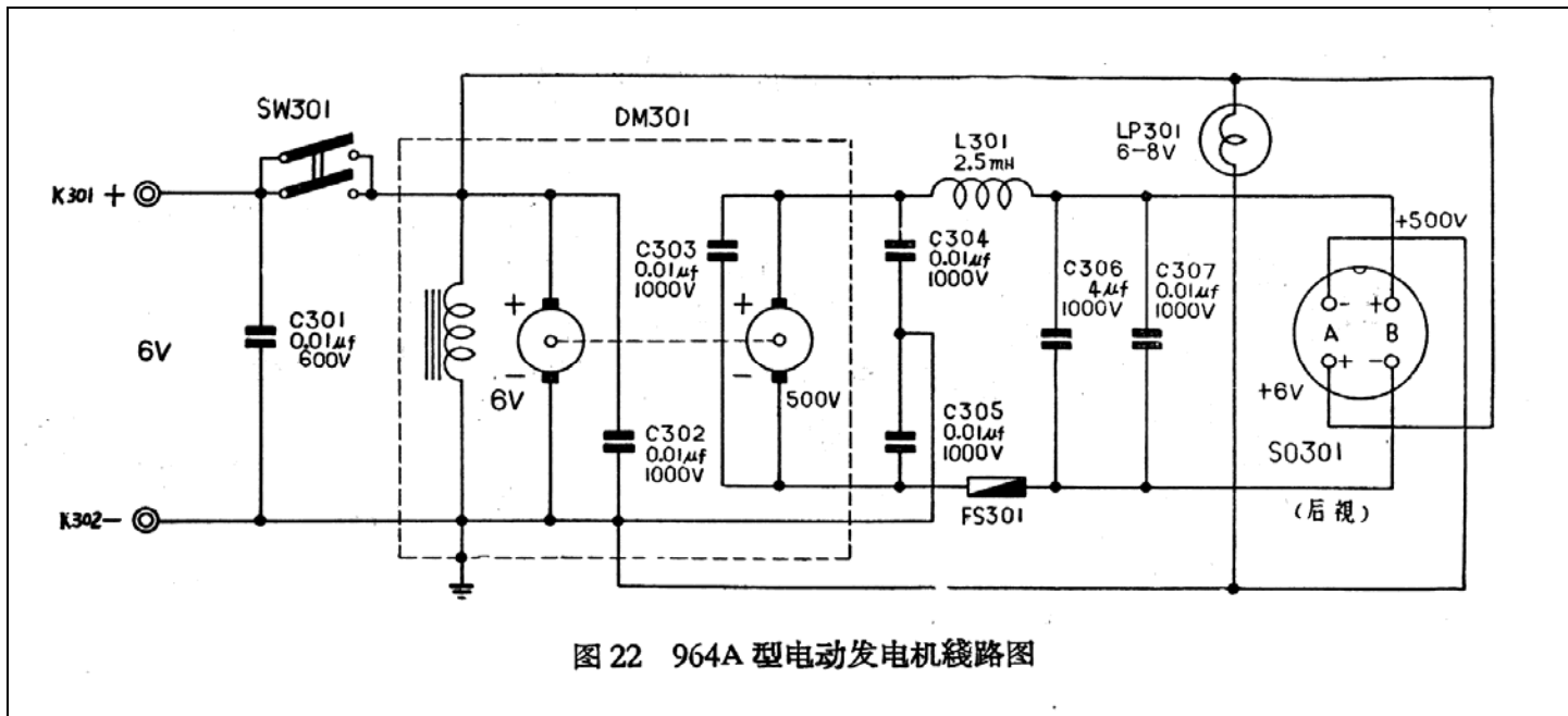
Figure 5: 6V Dynamotor
